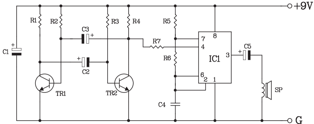
Figure 2. The train's whistle sound circuit
